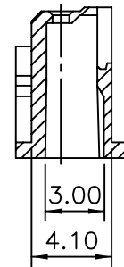
SECTION E-E
