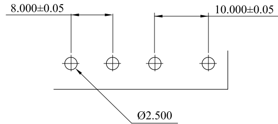
RECOMMENDED HOLE PATTERN
