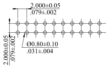
RECOMMENDED HOLE PATTERN
